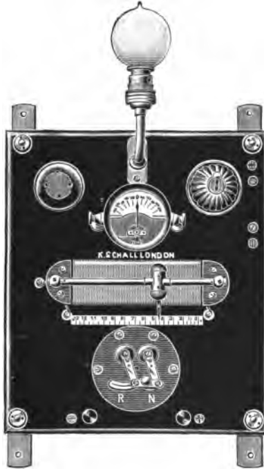
Switchboard for ionic medication.
